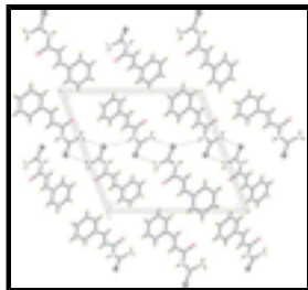
Fig. 2. Part of the crystal packing of (I), viewed down the b axis. Hydrogen bonds are shown as dashed lines.
